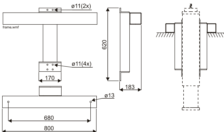
Figure 5: Suspension frame
