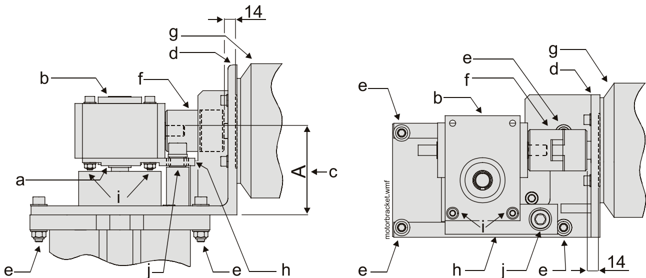
Figure 4: Installation of motor bracket
